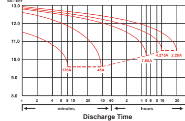
(h) Discharge Time VS. Discharge Current (25°C)
